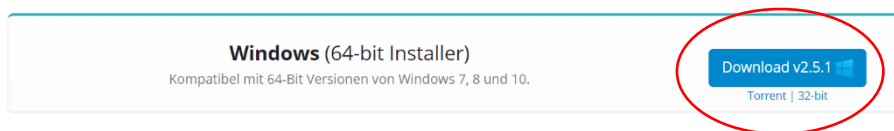
ABB.2, DOWNLOADBUTTON WINDOWSINSTALLER
